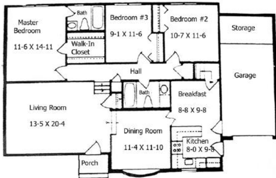
Upper Level
