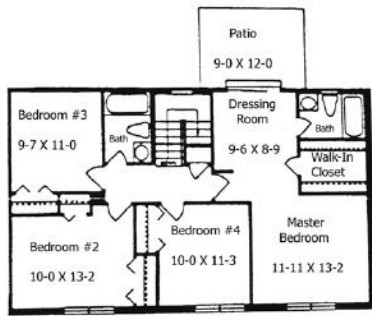
Second Level
